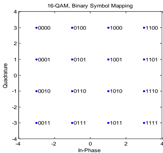
Fig. 6 Binary symbol mapping of 16-QAM
