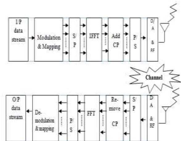
Fig. 2 Block diagram of an OFDM system
