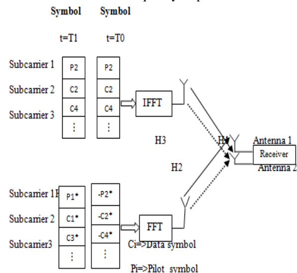
Fig. 3 Channel estimation for MIMO-OFDM systems
