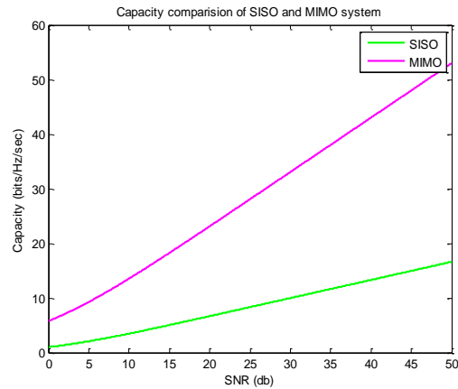
Fig. 4 Capacity vs. SNR for SISO/MIMO system
