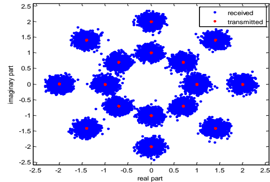
Fig. 7 Constellation diagram of 16-QAM
